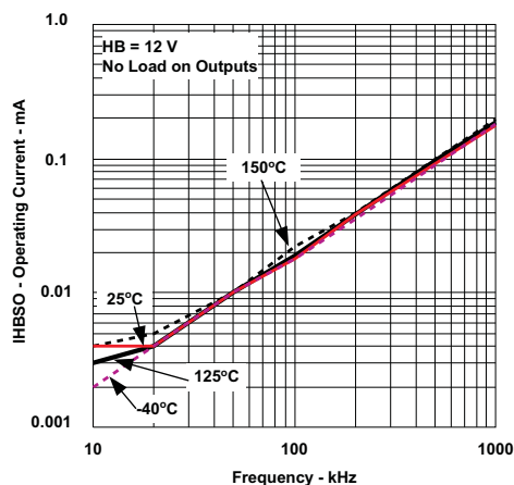
Figure 5. HB to VSS Operating Current vs Frequency
