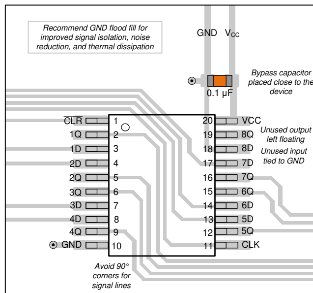
图 11-1. Example Layout for the SN74HCS273 PW package
