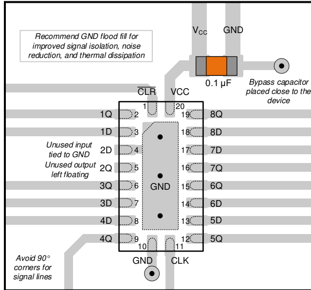
图 11-2. Example Layout for the SN74HCS273 RKS package
