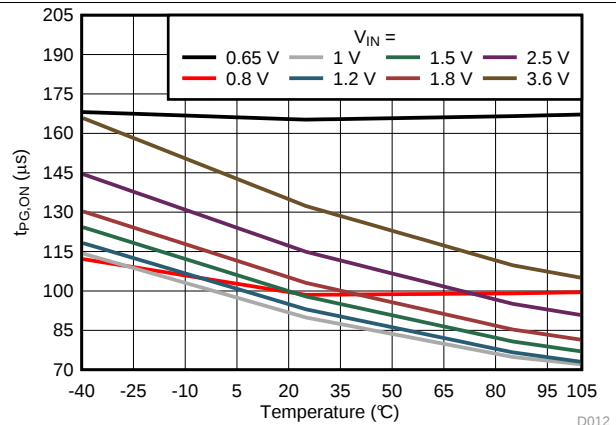
图 8. PG Turn-On Time vs Temperature
