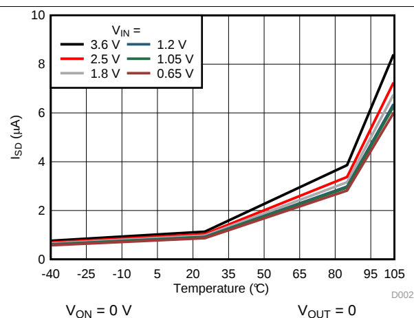
图 2. Input Shutdown Current vs Temperature
