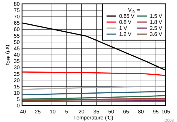
图 10. Turn-Off Time vs Temperature
