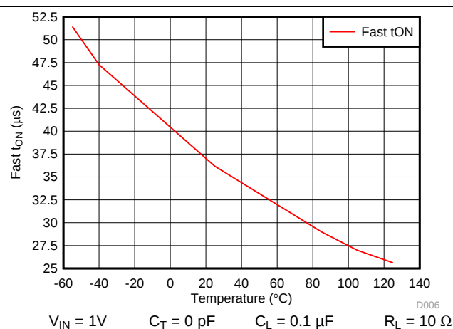
图 6. Fast Turn-On Time vs Temperature
