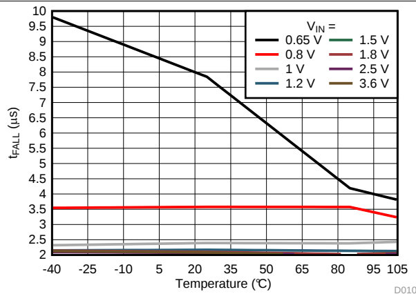
图 9. PG Turn-Off Time vs Temperature
