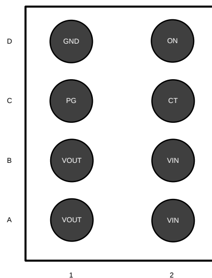
YZP Package 8-Pin DSBGA Bump View
