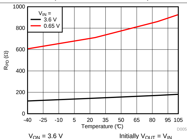
图 4. Output Pull-Down Resistance vs Temperature
