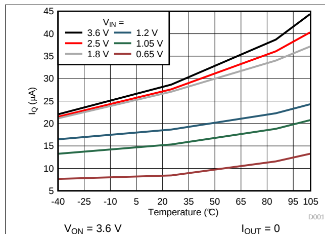
图 1. Quiescent Current vs Temperature
