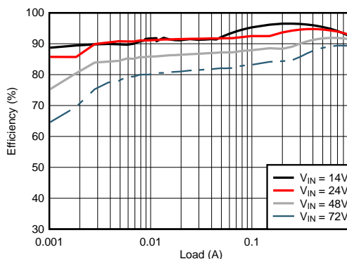
典型应用效率, V_{OUT} = 12\text{V}
