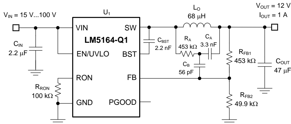
图 12. Typical Application V_{IN(nom)} = 48 V , V_{OUT} = 12 V , I_{OUT(max)} = 1 A , F_{SW(nom)} = 300 kHz
