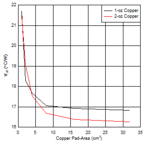
Figure 8-19. 4-Layer PCB Junction-to-Board Characterization (Ψ JB ) Parameter vs Copper Area
