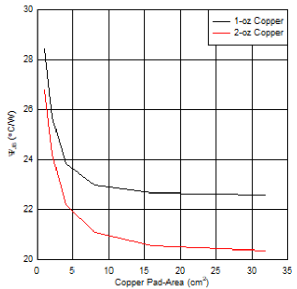
Figure 8-17. 2-Layer PCB Junction-to-Board Characterization Parameter (Ψ JB ) vs Copper Area
