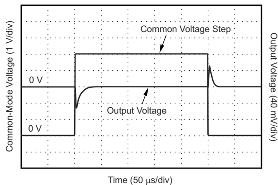
图 7-15. Common-Mode Voltage Transient Response
