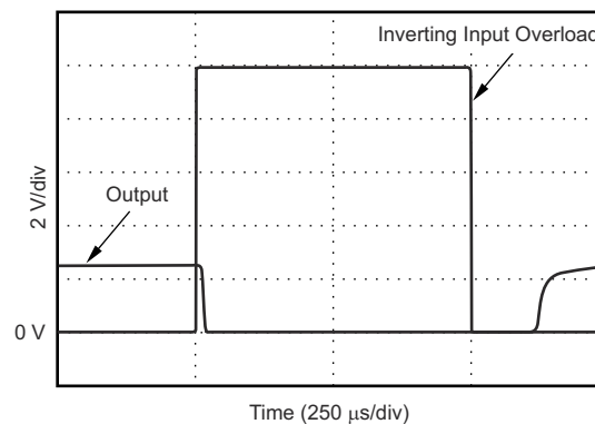
图 7-16. Inverting Differential Input Overload
