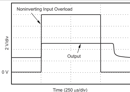
图 7-17. Noninverting Differential Input Overload
