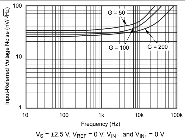
图 7-12. Input-Referred Voltage Noise vs. Frequency
