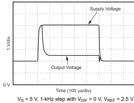
图 7-19. Brownout Recovery
