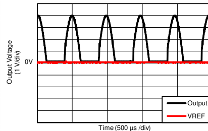
图 9-8. Unidirectional Application Output Response
