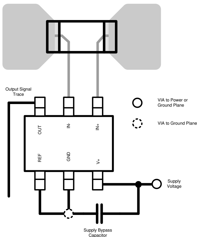
图 11-1. Recommended Layout
