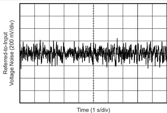
图 7-13. 0.1-Hz to 10-Hz Voltage Noise (Referred-to-Input)
