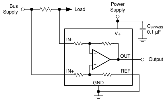
图 9-7. Unidirectional Application Schematic
