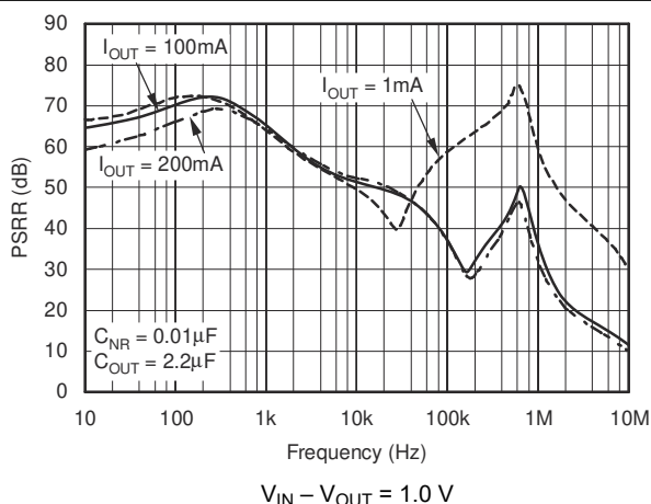
Figure 6-10. TPS799285 Power-Supply Ripple Rejection vs Frequency
