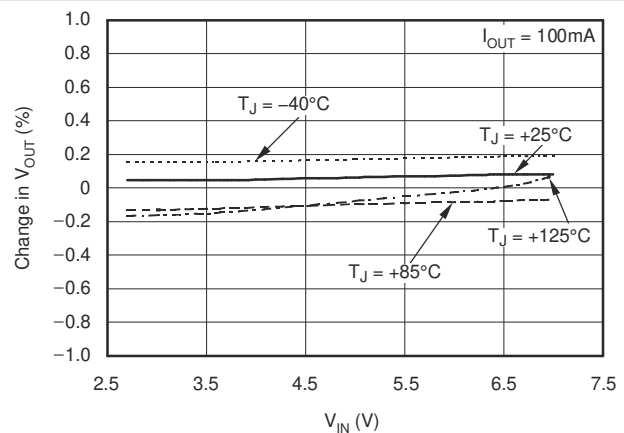
Figure 6-2. Line Regulation
