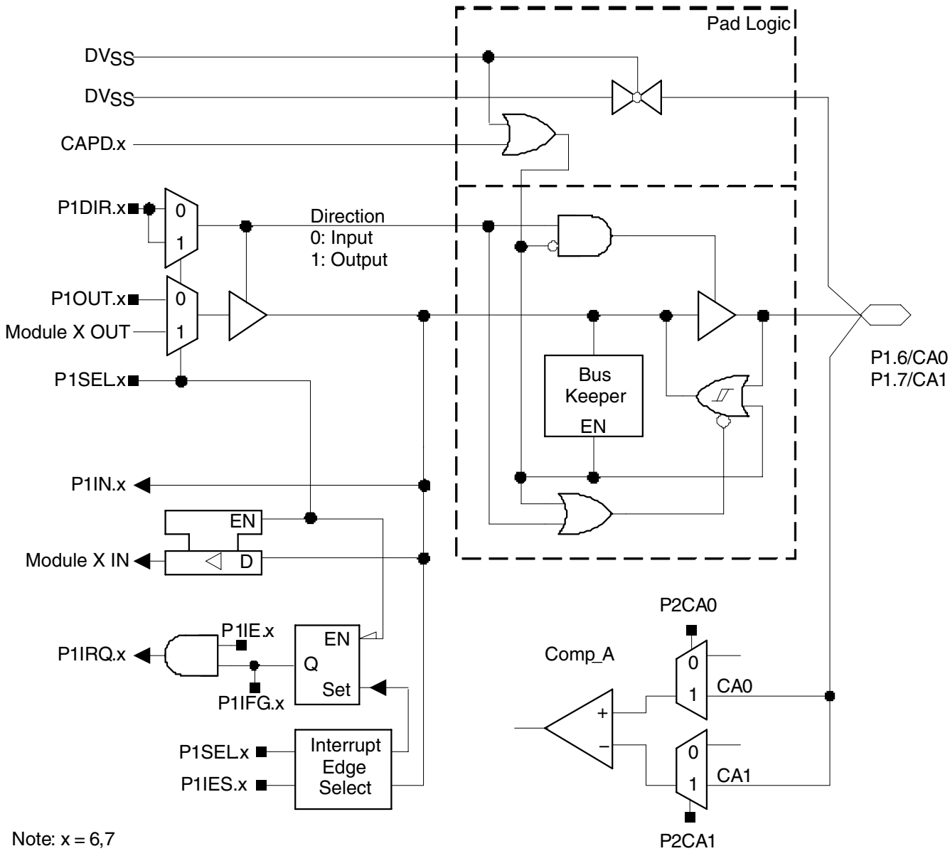
port P1 (P1.6 and P1.7) pin functions
