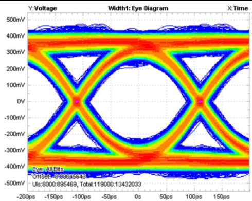
Figure 28. Eye Pattern: 4.5 Gbps With No Device
