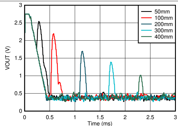
图 31. TUS4470 400 kHz Ranging at 20-V Driver
