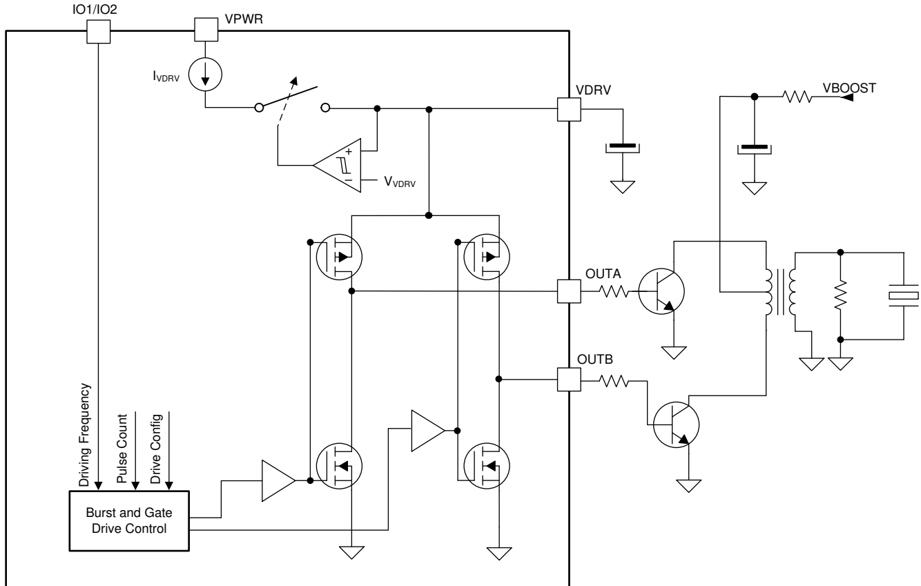
图 20. Center-Tap Transformer Drive Using External FETs
