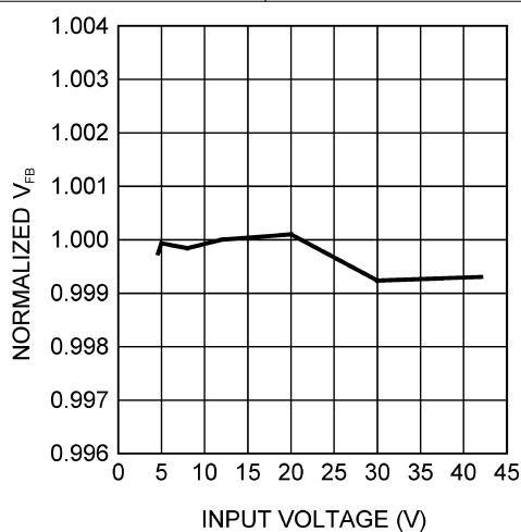
图 6-9. Normalized Feedback Voltage vs Input Voltage
