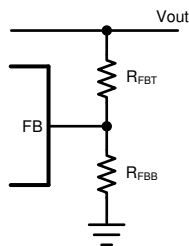
图 8-1. Resistive Feedback Divider
