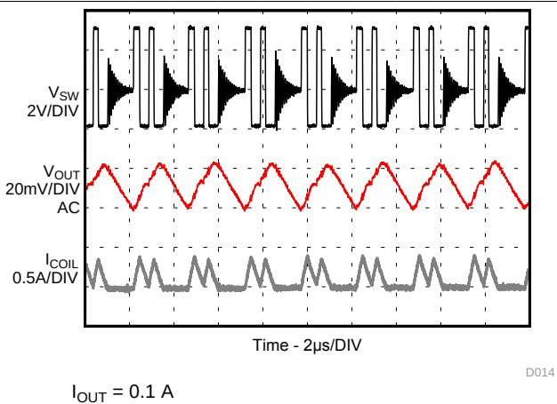
图 15. Power Save Mode Operation
