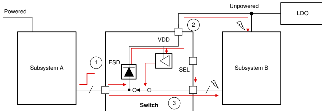
图 8-1. System Without Powered-Off Protection
