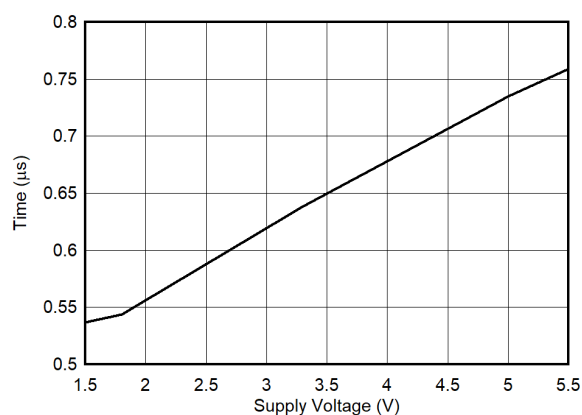
图 6-12. t_{\text{OFF\_VDD}} vs Supply Voltage
