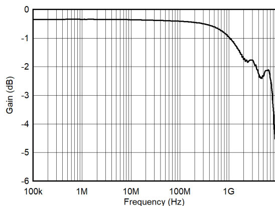
图 6-15. Differential Bandwidth
