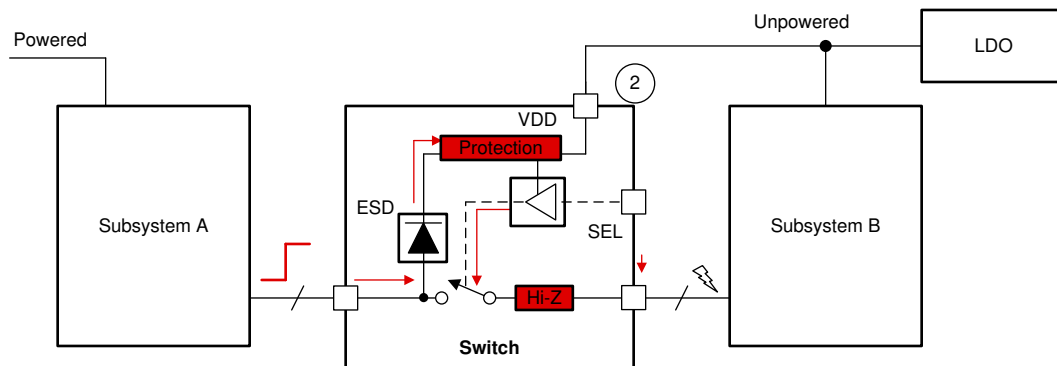
图 8-2. System With Powered-Off Protection
