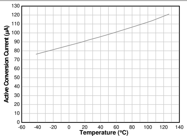
Figure 6-9. Active Conversion Current vs. Temperature
