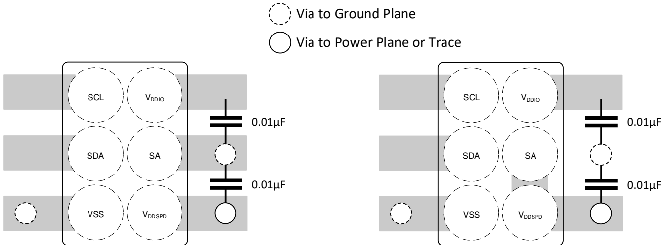
Figure 10-1. Layout Example
