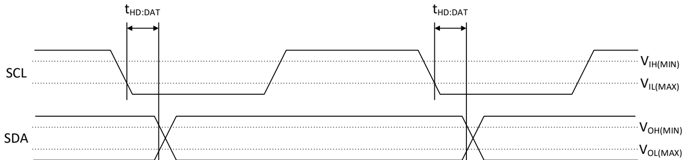
Figure 6-4. I 2 C Basic Bus Output Timing Diagram
