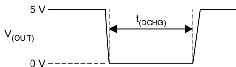
图 9-3. OUT Discharge During Mode Change
