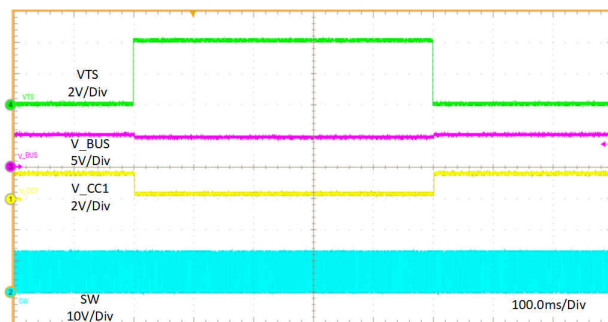
图 11-27. OUT Hot Short to GND
