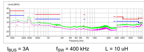
图 11-5. 400-KHz EMI Results (Without CM Filter)
