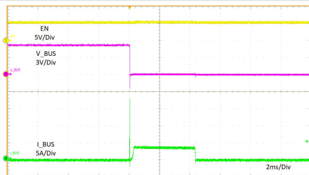
图 11-24. VBUS Hot Short to GND
