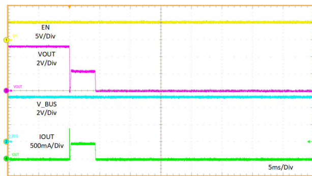
图 11-26. OUT short to 5.1- \Omega Load
