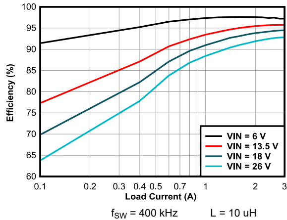
图 11-2. Buck Only Efficiency
