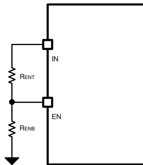
图 10-1. System UVLO by Enable Divider
