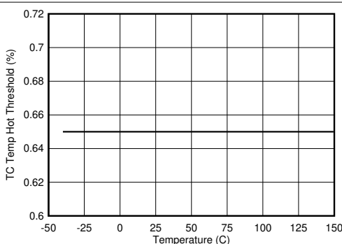
图 8-23. TS Temperature Hot Threshold vs Junction Temperature
