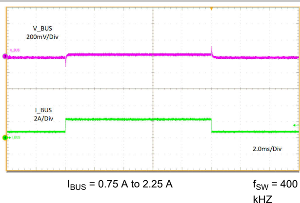
图 11-11. Load Transient With Cable Compensation
