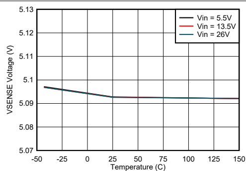
图 8-4. V_{SENSE} Voltage vs Junction Temperature
