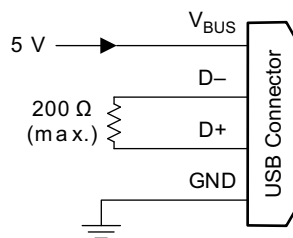
图 10-15. DCP Supporting BC1.2 and YD/T 1591-2009
