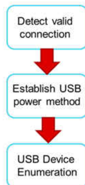
图 10-13. Flow of DFP to UEP Configuration
