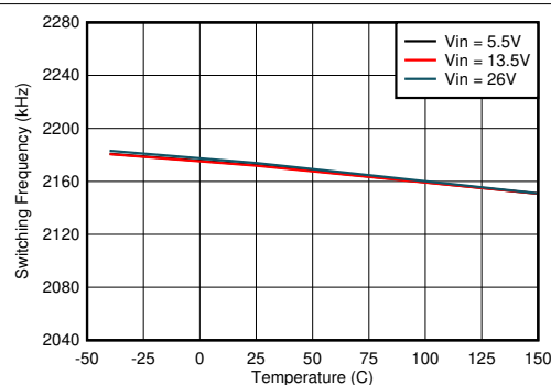
图 8-20. Switching Frequency vs Junction Temperature
