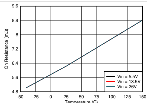
图 8-16. USB Power Switch On Resistance vs Junction Temperature
