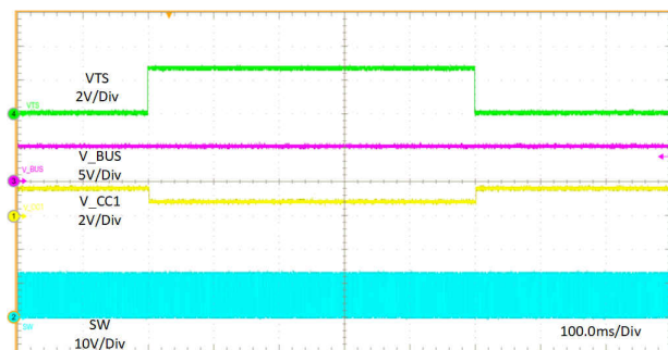
图 11-26. OUT short to 5.1- \Omega Load
