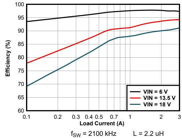
图 11-3. Buck Only Efficiency
