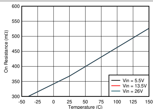
图 8-18. V_{CONN} Power Switch On Resistance vs Junction Temperature
