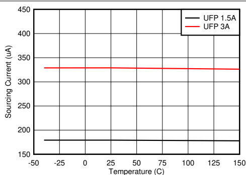
图 8-21. CC Sourcing Current vs Junction Temperature
