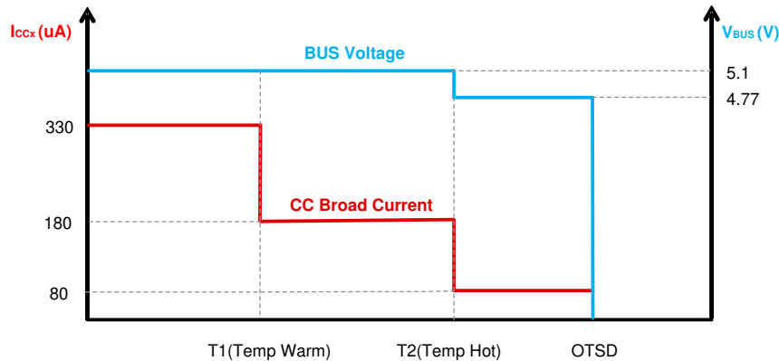
图 10-11. TPS2585x-Q1 Behavior When Trigger Temp Warm/Hot Threshold
