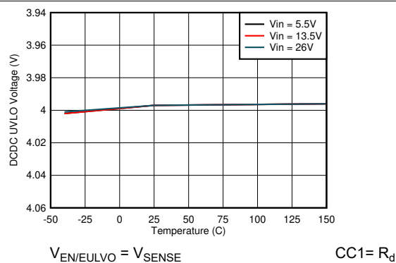
图 8-5. DCDC UVLO Threshold
