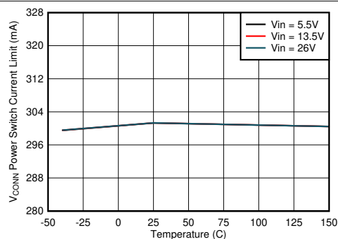
图 8-14. V_{CONN} Power Switch Current Limit vs Junction Temperature
