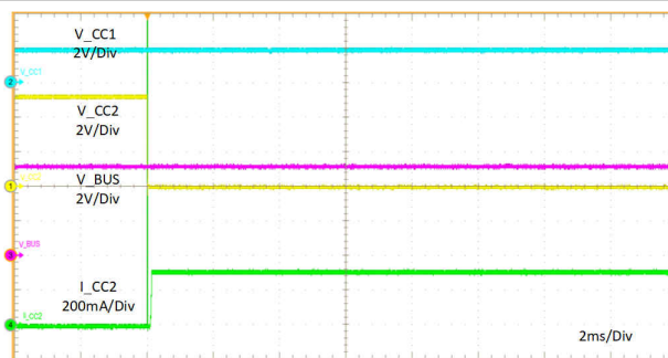
图 11-23. Short Circuit Recovery
