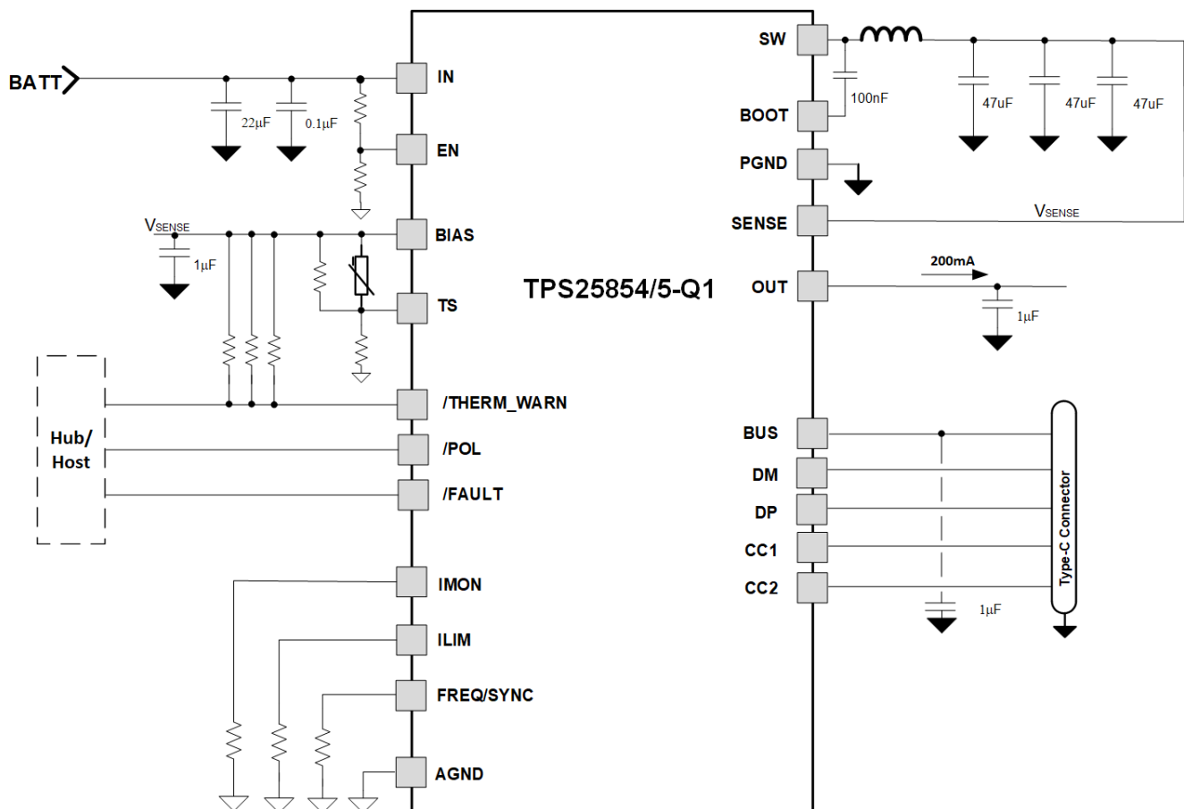
图 11-1. TPS2585x-Q1 Typical Application Circuit for 400-KHz f_{sw}
