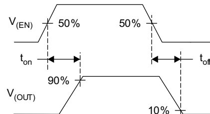
图 9-4. Enable Timing, Active-High Enable
