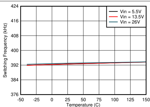
图 8-19. Switching Frequency vs Junction Temperature
