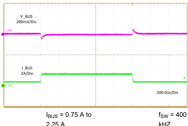
图 11-9. Load Transient Without Cable Compensation
