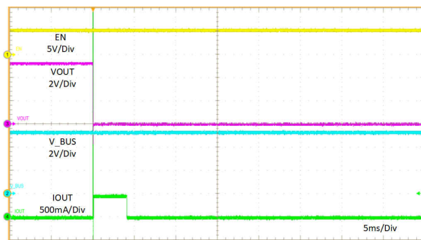
图 11-27. OUT Hot Short to GND
