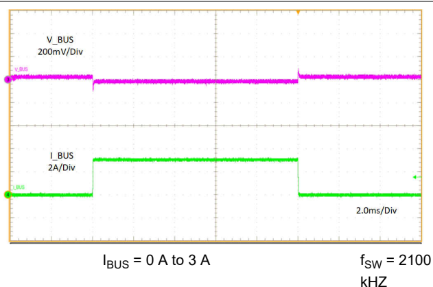
图 11-10. Load Transient With Cable Compensation
