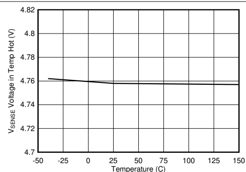
图 8-24. SENSE Voltage in Temperature Hot vs Junction Temperature
