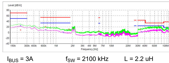
图 11-4. 2.1-MHz EMI Results (Without CM Filter)
