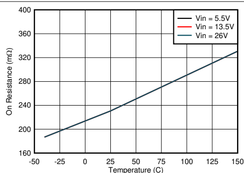
图 8-17. OUT Power Switch On Resistance vs Junction Temperature
