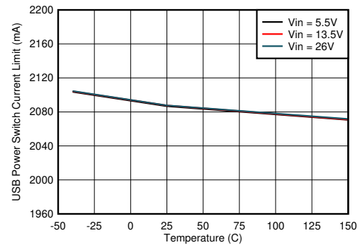
图 8-10. USB Power Switch Current Limit vs Junction Temperature
