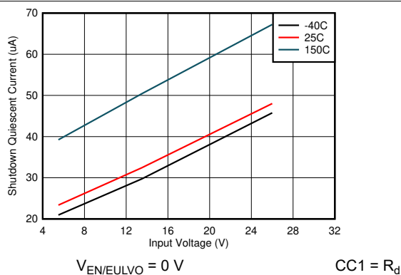
图 8-1. Shutdown Quiescent Current
