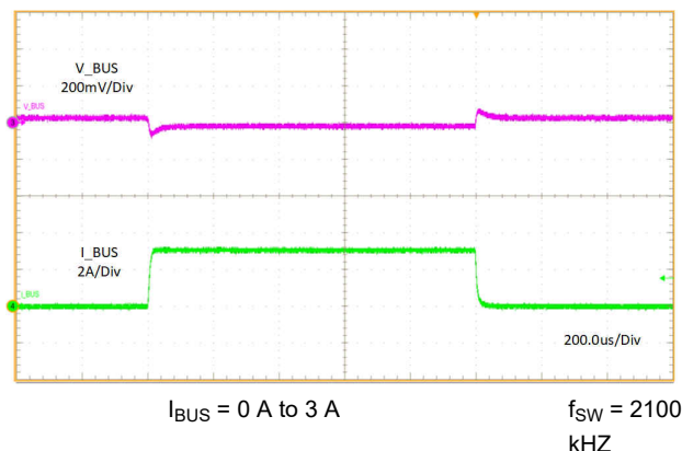
图 11-8. Load Transient Without Cable Compensation
