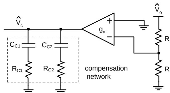
Figure 19. Compensation Network
