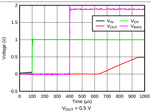
图 24. Startup With V_{BIAS} Powering Up After V_{IN} and V_{EN}
