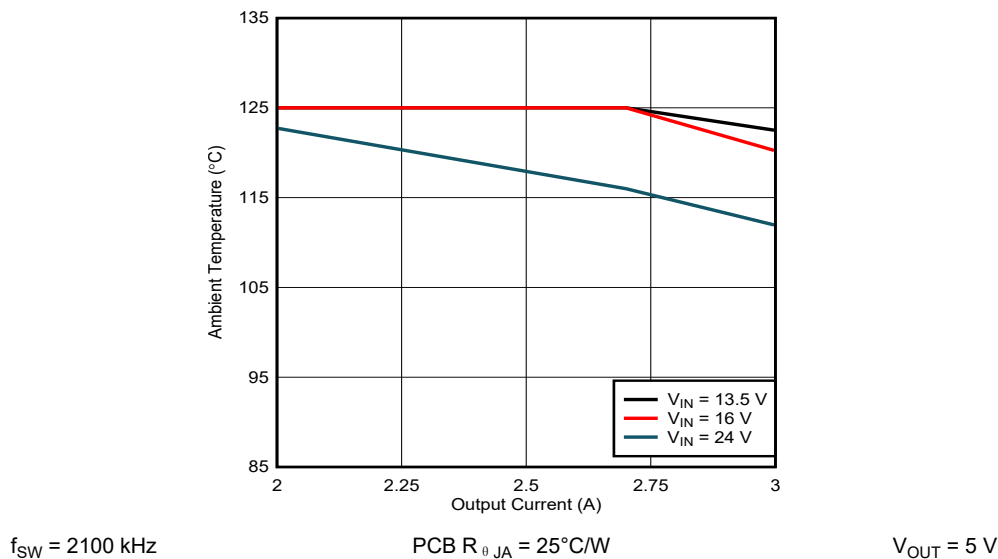
图 9-2. Maximum Ambient Temperature versus Output Current
