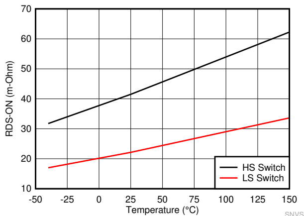
图 7-5. High-Side and Low-Side Switches R_{DS\_ON}
