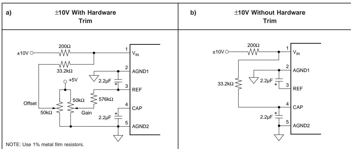
FIGURE 6. Circuit Diagram With and Without External Resistors.
