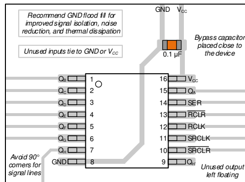
图 11-1. Example layout for the SN74HCS594-Q1 in the PW package.
