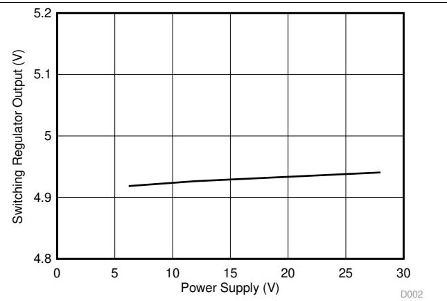
Figure 6. Step-Down Regulator Output vs Power Supply Voltage
