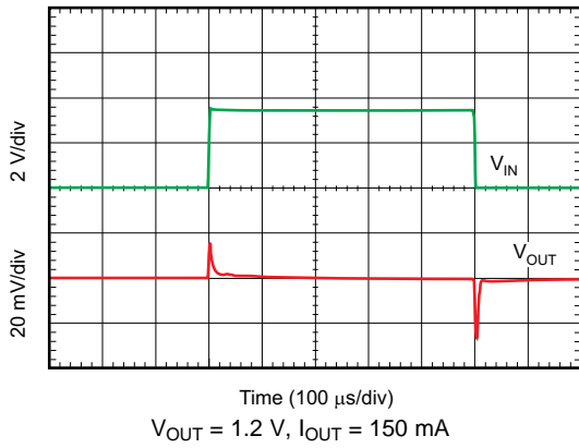
图 35. Line Transient Response
