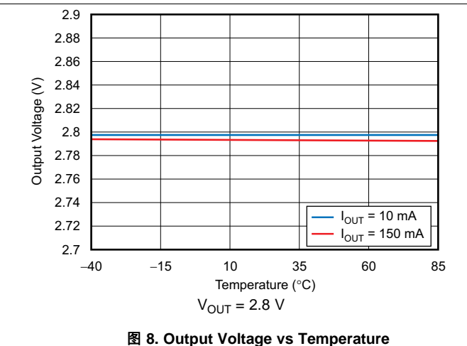
图 8. Output Voltage vs Temperature
