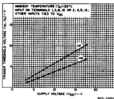
Fig. 12 - Typical trigger threshold voltage vs. V_{DD} .
