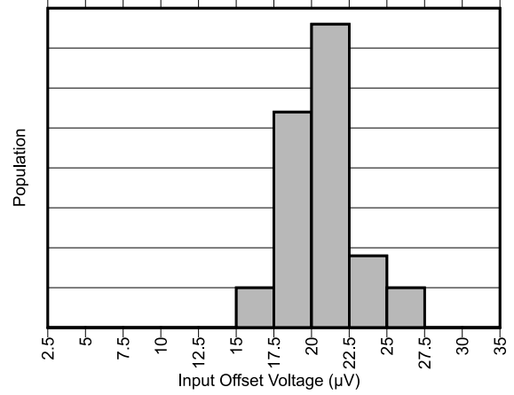
图 6-6. Input Offset Production Distribution, A1 Devices (INA4290)
