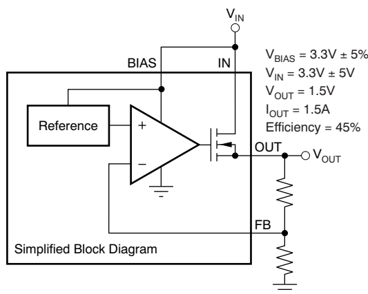
Figure 25. Typical Application of the TPS742 Without an Auxiliary Bias
