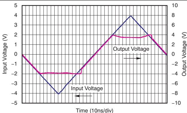
Figure 25. Noninverting Overdrive Recovery
