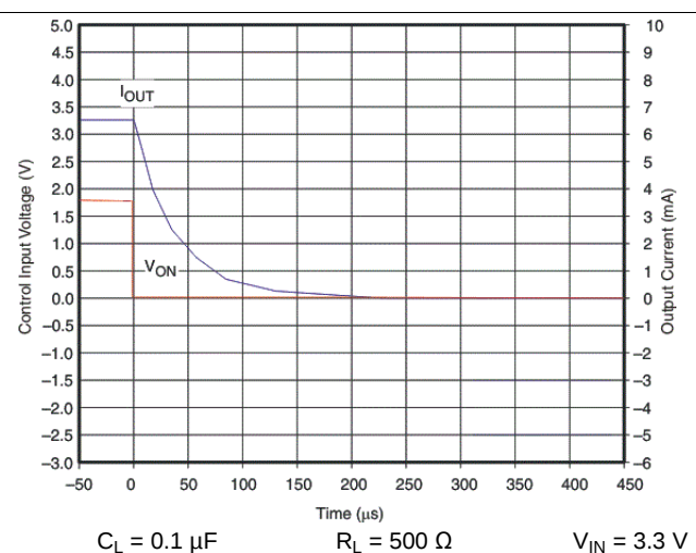
Figure 23. t_{ON} Response
