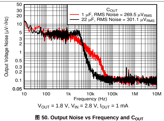
图 50. Output Noise vs Frequency and C_{OUT}
