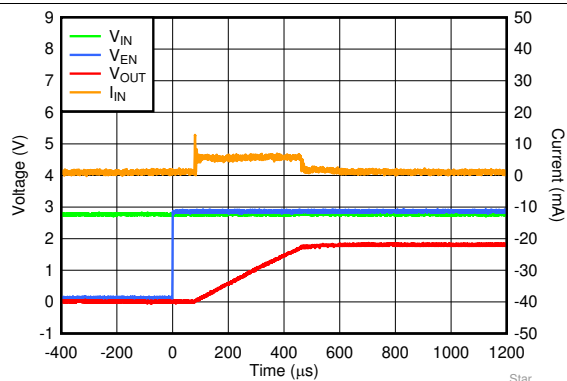
图 56. Startup Inrush Current With C_{OUT} = 1\text{ }\mu\text{F}
