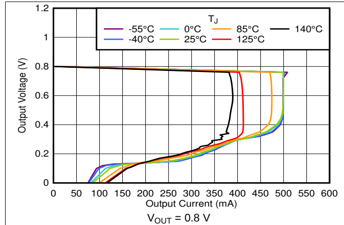
图 37. Foldback Current Limit vs I_{OUT} and Temperature
