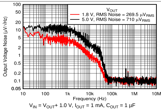
图 48. Output Noise vs Frequency and V_{OUT}
