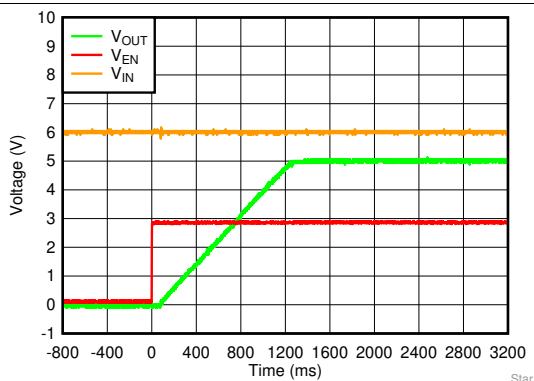
图 55. Startup With V_{EN} After V_{IN}
