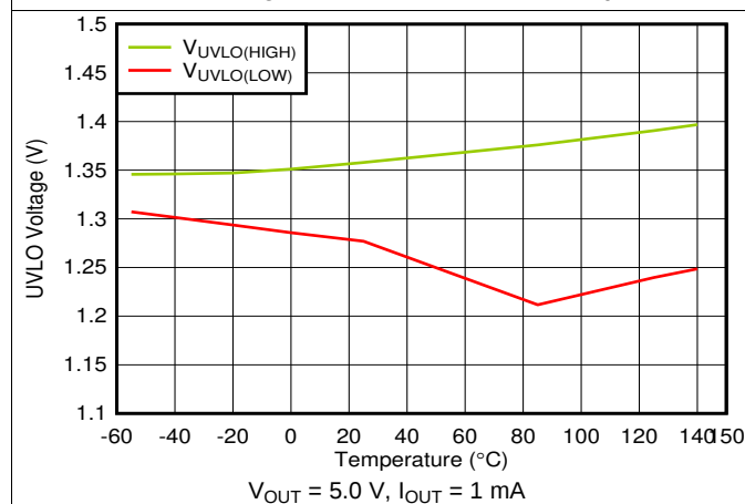
图 41. UVLO Rising and Falling Threshold vs Temperature
