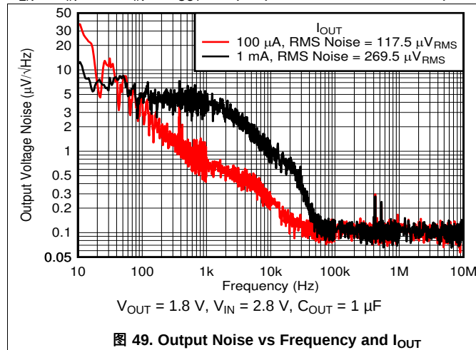
图 49. Output Noise vs Frequency and I_{OUT}
