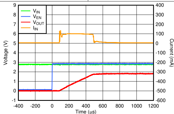
图 55. Startup With V_{EN} After V_{IN}
