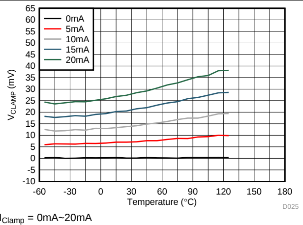
图 24. UCC5310M V_{Clamp} vs Temperature
