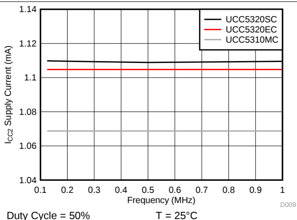
图 20. I_{CC2} Supply Current vs Input Frequency
