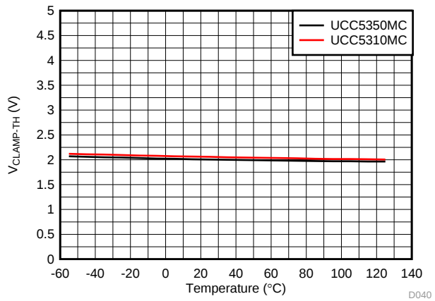
图 24. UCC5310M V_{Clamp} vs Temperature
