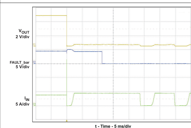
图 10-6. Full-Load to Short-Circuit Transient Response
