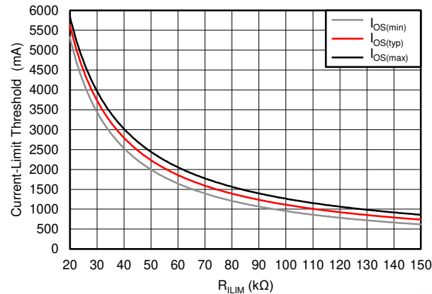
图 10-2. Current-Limit Threshold versus R_{(ILIM)}
