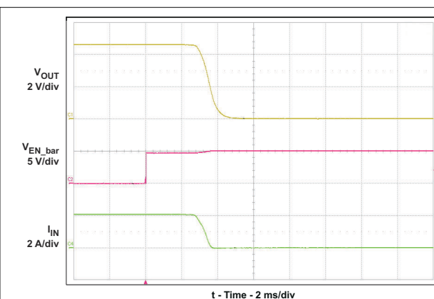
图 10-4. Turnoff Delay and Fall Time
