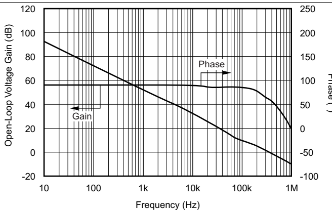
Figure 2. Open-Loop Gain vs Frequency
