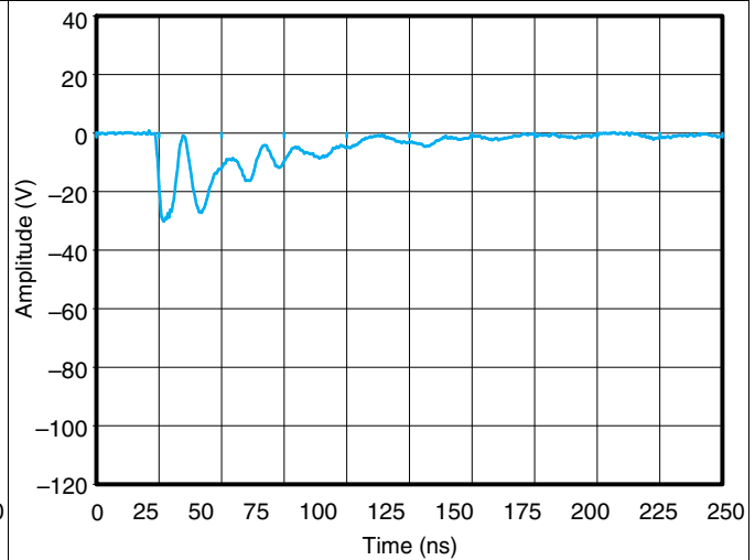
Figure 10. V_{BUS} IEC Clamping Waveform, -8 kV Contact, 25 ns/div
