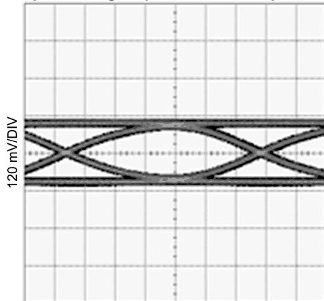
25 ps/DIV Figure 14.
