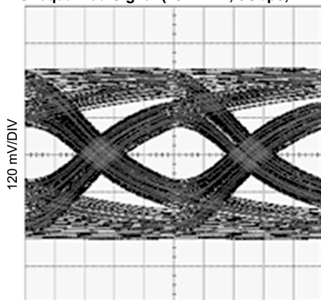
40 ps/DIV Figure 10.
