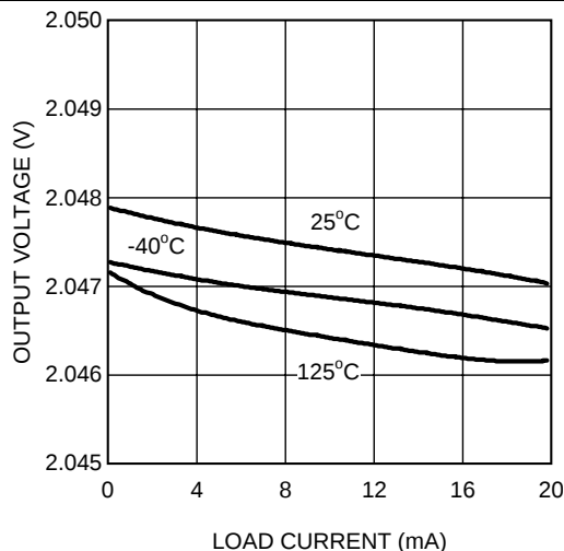
Figure 18. Load Regulation
