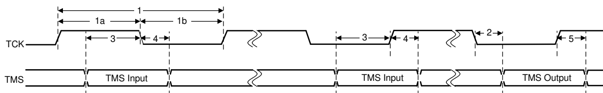
图 7-20. cJTAG Timing
