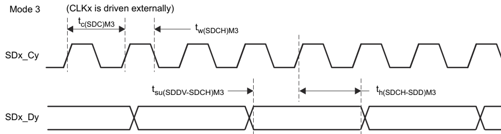
图 7-68. SDFM Timing Diagram - Mode 3
