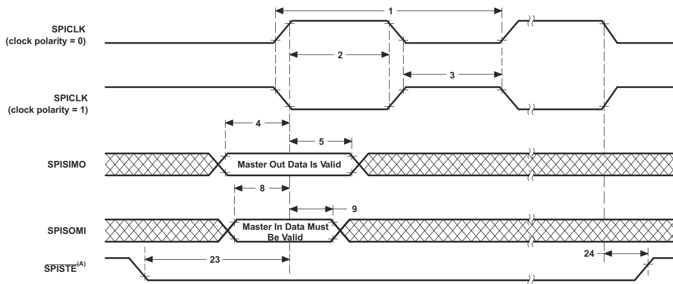
图 7-80. High-Speed SPI Master Mode External Timing (Clock Phase = 1)
