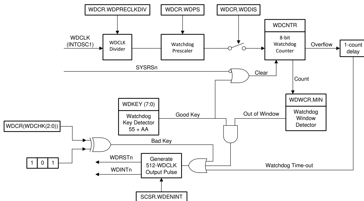
图 8-4. Windowed Watchdog
