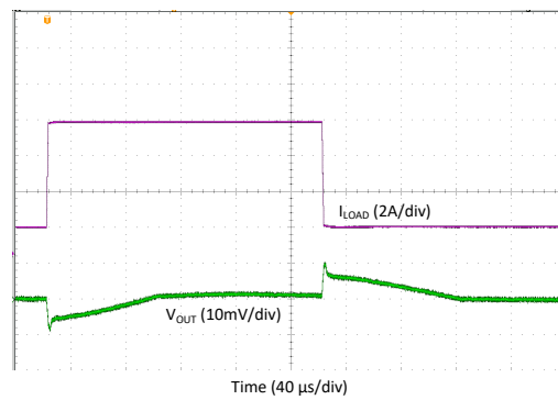
图 8-15. Transient Load Step Response, Forced-PWM-Four-Phase Mode, T_A = -40^\circ\text{C}
