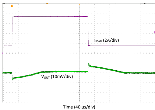
图 8-14. Transient Load Step Response, Forced-PWM-Four-Phase Mode, T_A = +25^\circ\text{C}
