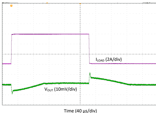
图 8-14. Transient Load Step Response, Forced-PWM-Four-Phase Mode, T_A = +25^\circ\text{C}
