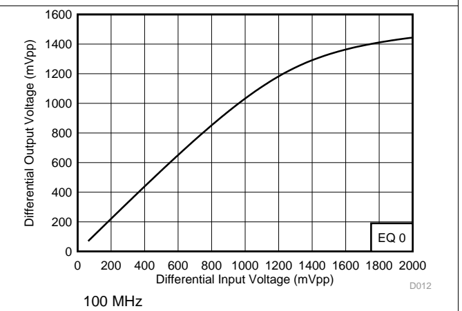
图 18. Upstream-to-Downstream Linearity Performance at 100 MHz
