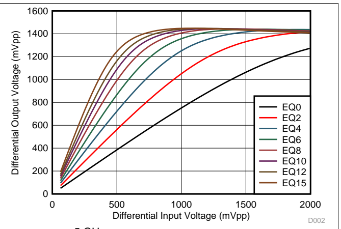
图 16. Upstream-to-Downstream Linearity Performance at 5 GHz
