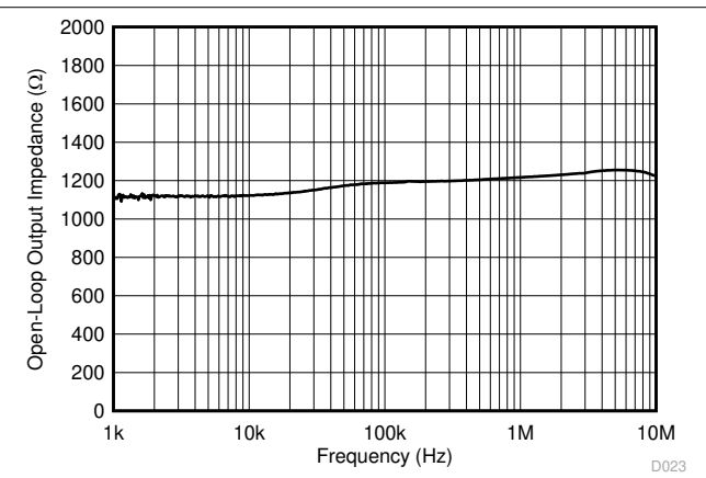
图 6-18. Open-Loop Output Impedance vs Frequency
