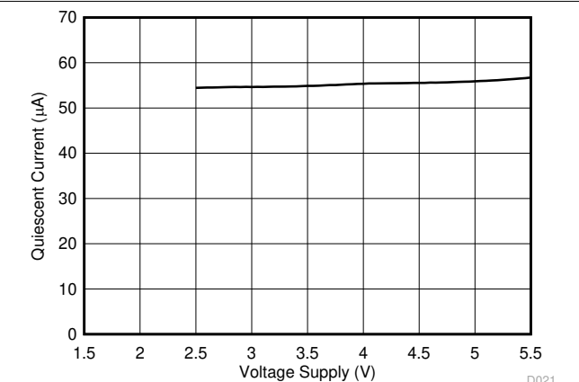
图 6-16. Quiescent Current vs Supply Voltage
