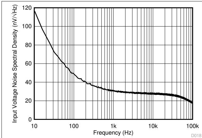
图 6-13. Input Voltage Noise Spectral Density
