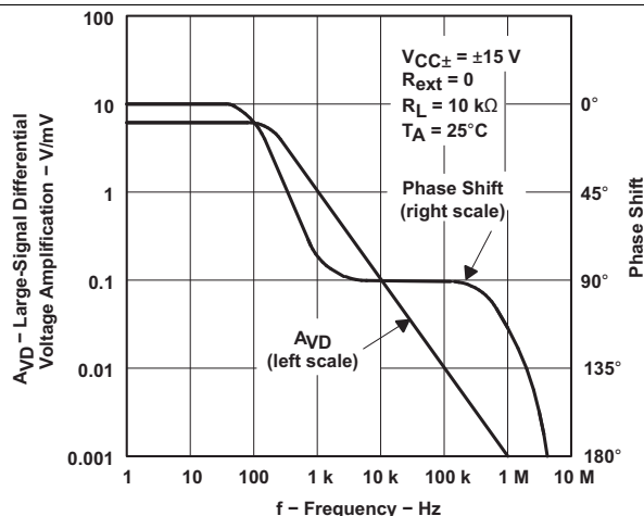
Figure 6. Large-Signal Differential Voltage Amplification and Phase Shift vs Frequency
