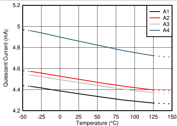
图 7-14. Quiescent Current vs. Temperature
