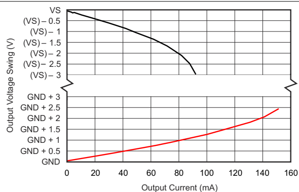
图 7-12. Output Swing vs. Output Current
