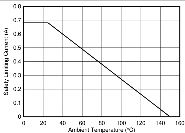
图 7-23. Thermal Derating Curve for Safety-Limiting Current, Side 2
