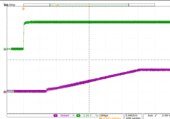
图 10-53. Start-Up Timing
