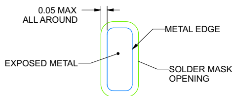
NON SOLDER MASK DEFINED SOLDER MASK DETAIL
