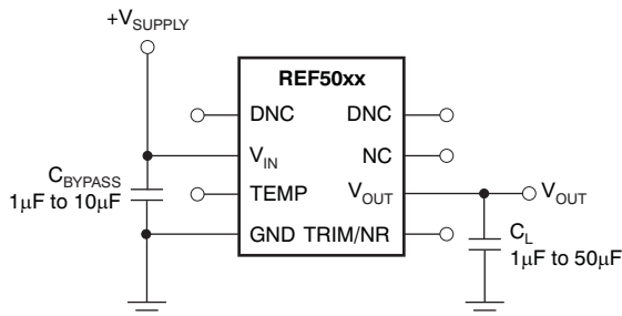
Figure 42. Basic Connections
