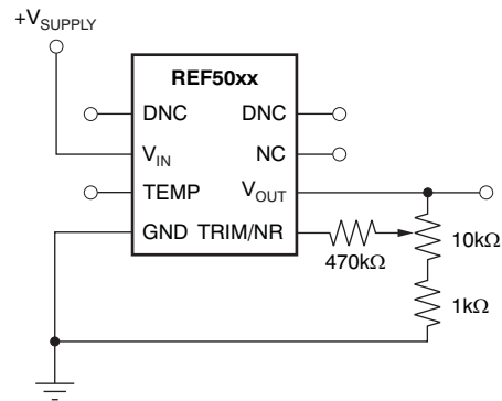
Figure 41. V_{OUT} Adjustment Using the TRIM/NR Pin
