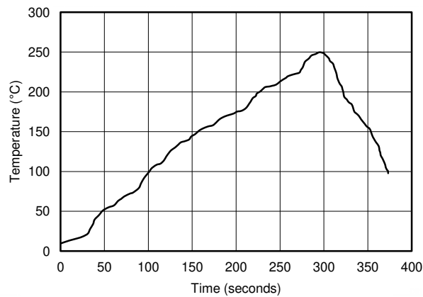
Figure 30. Reflow Profile
