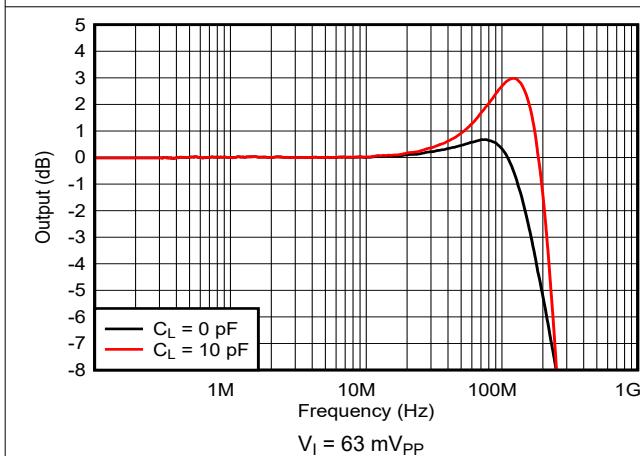
Figure 7-5. Small-Signal Frequency Response
