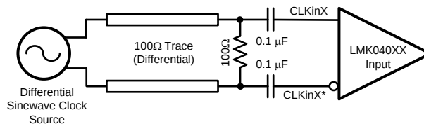
Figure 29. CLKInX/X* Termination for a Differential Sinewave Reference Clock Source
