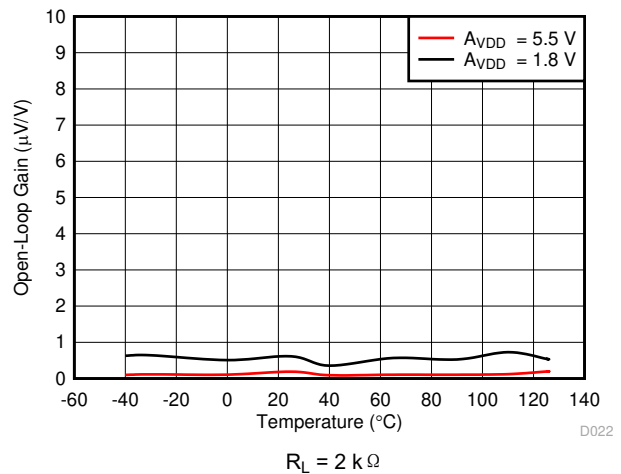
图 7-22. Open-Loop Gain vs Temperature
