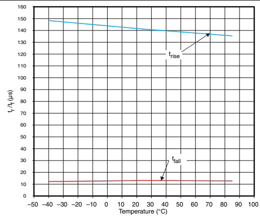
Figure 16. t rise /t fall vs Temperature (V IN = 3.3 V)
