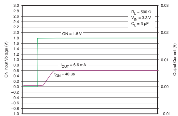
Figure 18. t ON Response
