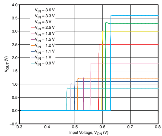
Figure 10. ON-Input Threshold
