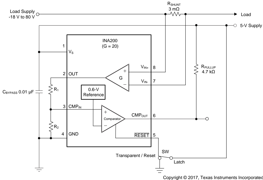
图 26. INA200 Basic Connections
