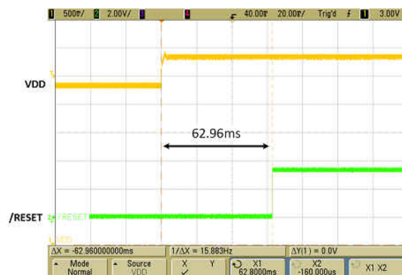
Figure 9-4. Reset Delay
