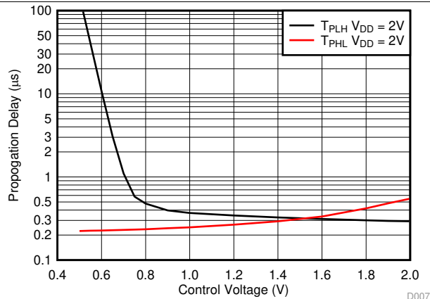
Figure 7. Propagation Delay vs Control Voltage V_{DD} = 2V
