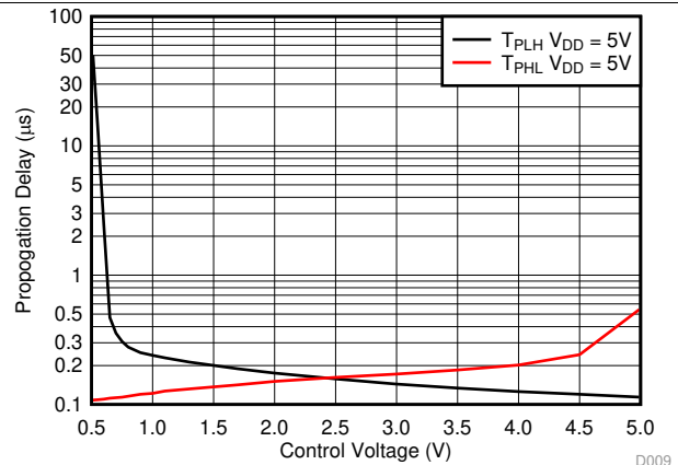
Figure 8. Propagation Delay vs Control Voltage V_{DD} = 5V
