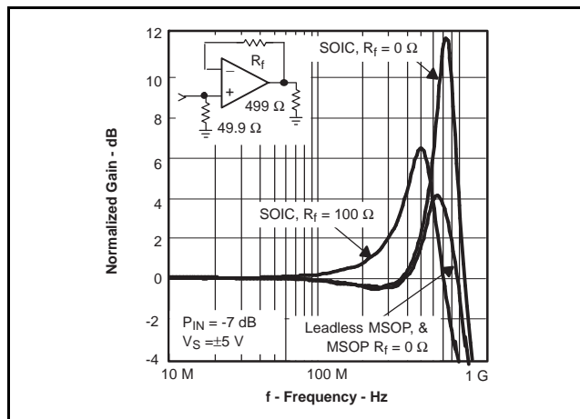
Figure 92. Effects of Unity-Gain Frequency Response for Differential Packages
