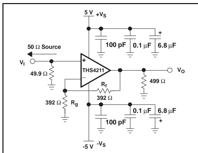
Figure 75. Wideband, Noninverting Gain Configuration
