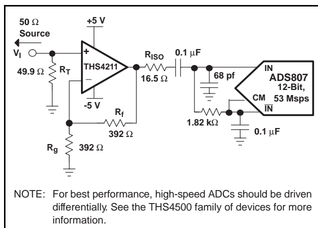
Figure 79. Driving an ADC With a Single-Ended Input
